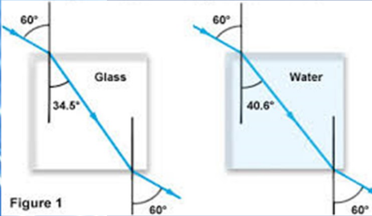
Light refraction through glass and water
